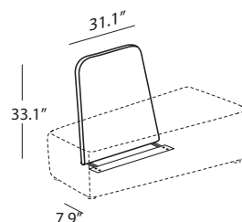
LOW BACKREST
