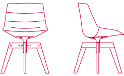
4-legged oak base L55 D57.5 H80.5 cm seat H44 cm armrest H68 cm
