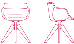
VN 4-legged oak base L57.5 D59 H76.4 cm seat H44 cm armrest H68 cm
