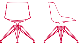
LEM 4-legged base L65 D65 H80.5 cm seat H44 cm
