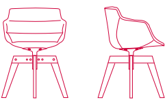
4-legged oak base L56 D58 H76.4 cm seat H44 cm armrest H68 cm
