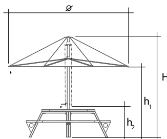
product dimensions (ft inch)
