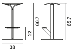
swivel version H67.5
