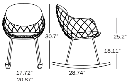
Rocking Chair
