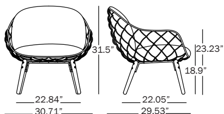
Low Armchair
