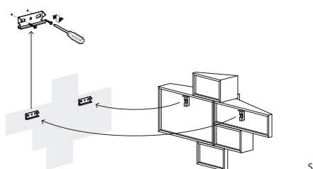
Assembly system
