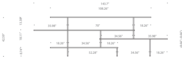
COMPOSITION C: L 108.26" H 37.87" D 15.74"
