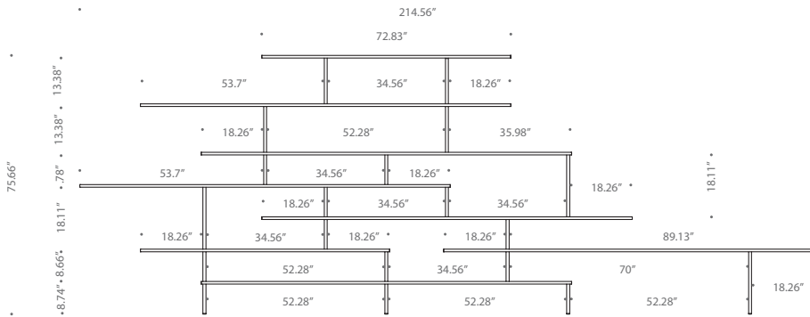
COMPOSITION B: L 143.7" H 42.59" D 15.74"
