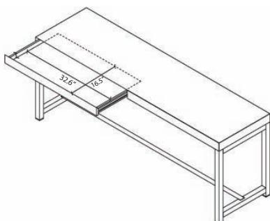
WRITING DESK WITH 2 DRAWERS 70.9"
